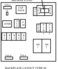
BACKPLATE LAYOUT TYPICAL
