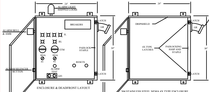
ENCLOSURE & DEADFRONT LAYOUT
