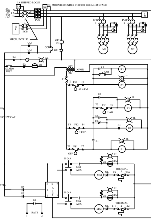
ELECTRICAL CONTROL PANEL SCHEMATIC FOR COMMERCIAL DUPLEX GRINDER PUMP 1PHASE
