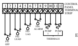
CONTROL PANEL TERMINAL STRIP
