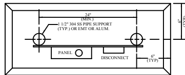
PLAN VIEW ELECTRICAL PANEL & CONCRETE PAD
