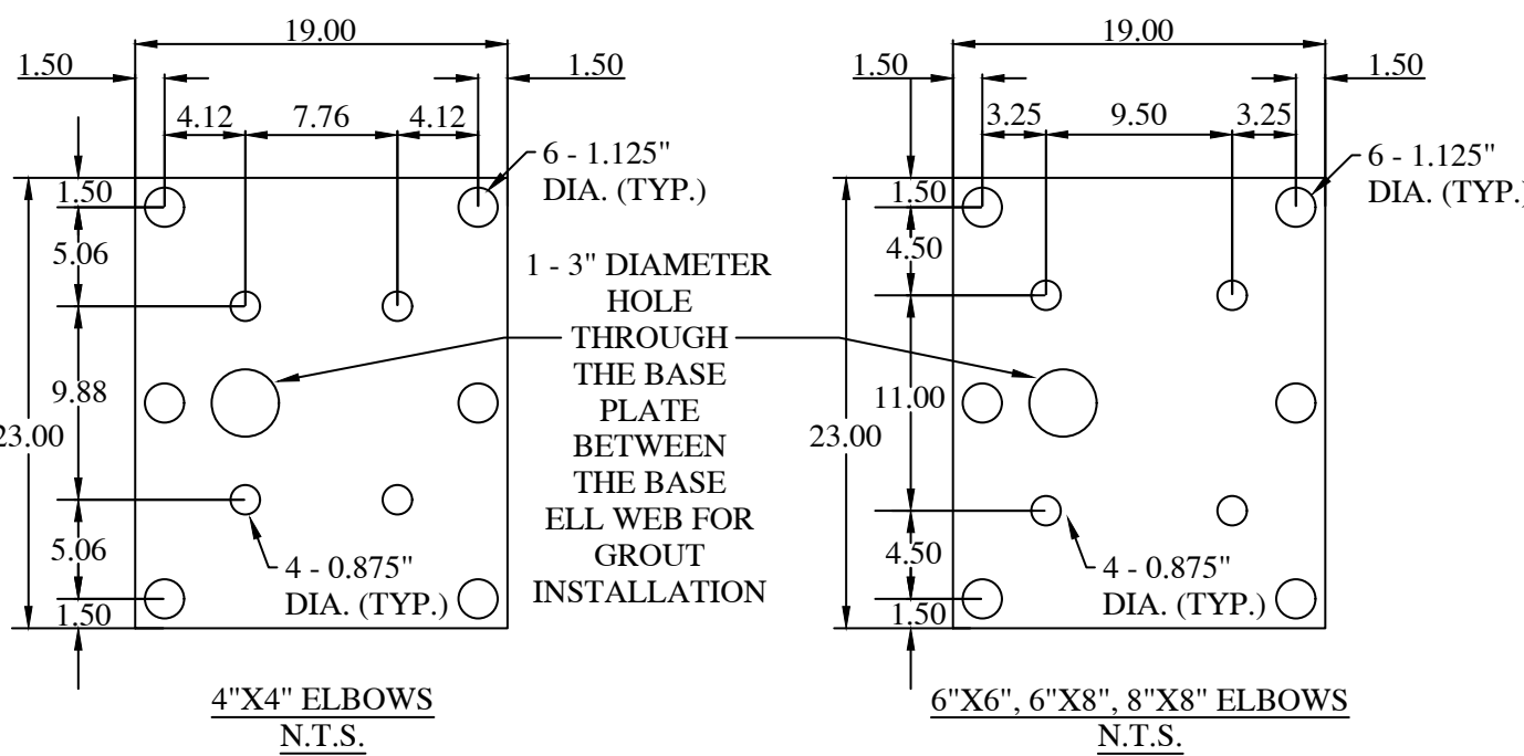
BASE PLATE: 316 STAINLESS STEEL 0.50" THICK (ALL MEASUREMENTS IN INCHES)
