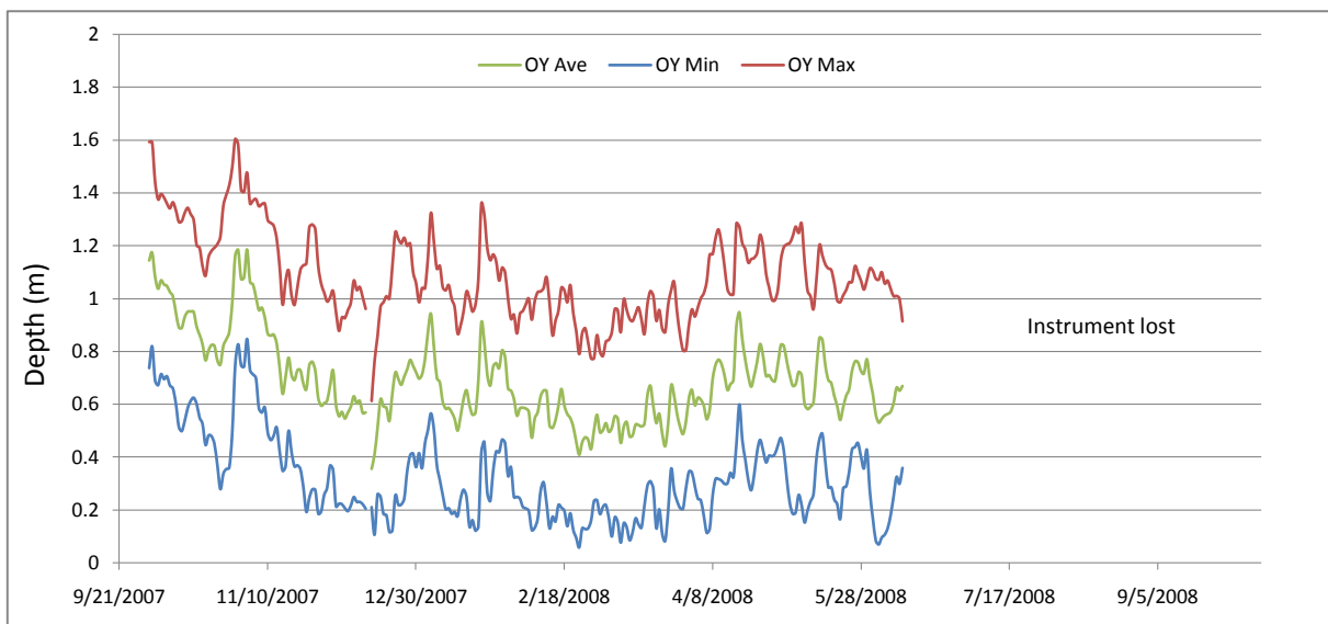
Station Oyster (OY) daily average, minimum, and maximum of water quality parameters measured by Datasonde recording at 15 minute intervals, Loxahatchee River, Florida. Data not meeting quality control criteria excluded.
