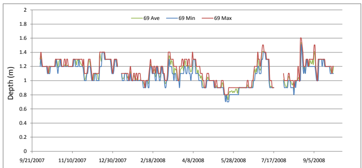
Station 69 daily average, minimum, and maximum of water quality parameters measured by Datasonde recording at 1 hour intervals, Loxahatchee River, Florida. Data not meeting quality control criteria excluded.
