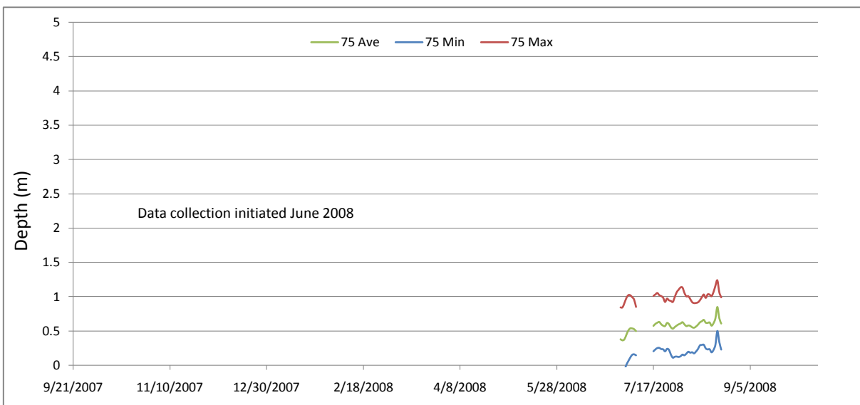
Station 75 daily average, minimum, and maximum of water quality parameters measured by Datasonde recording at 15 minute intervals, Loxahatchee River, Florida. Data not meeting quality control criteria excluded.
