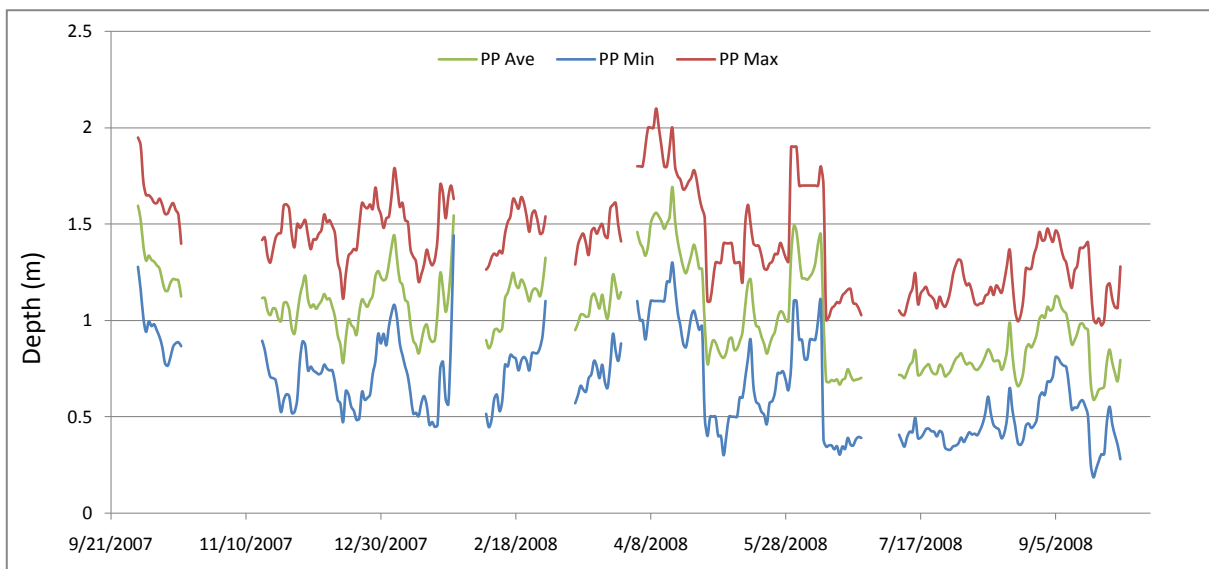
Station Pennock Point (PP) daily average, minimum, and maximum of water quality parameters measured by Datasonde recording at 15 minute intervals, Loxahatchee River, Florida. Data not meeting quality control criteria excluded.
