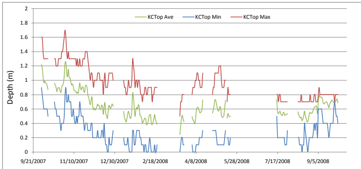
Station Kitching Creek (Surface) daily average, minimum, and maximum of water quality parameters measured by Datasonde recording at 15 minute intervals, Loxahatchee River, Florida. Data not meeting quality control criteria excluded.
