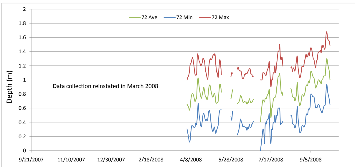
Station 72 daily average, minimum, and maximum of water quality parameters measured by Datasonde recording at 15 minute intervals, Loxahatchee River, Florida. Data not meeting quality control criteria excluded.
