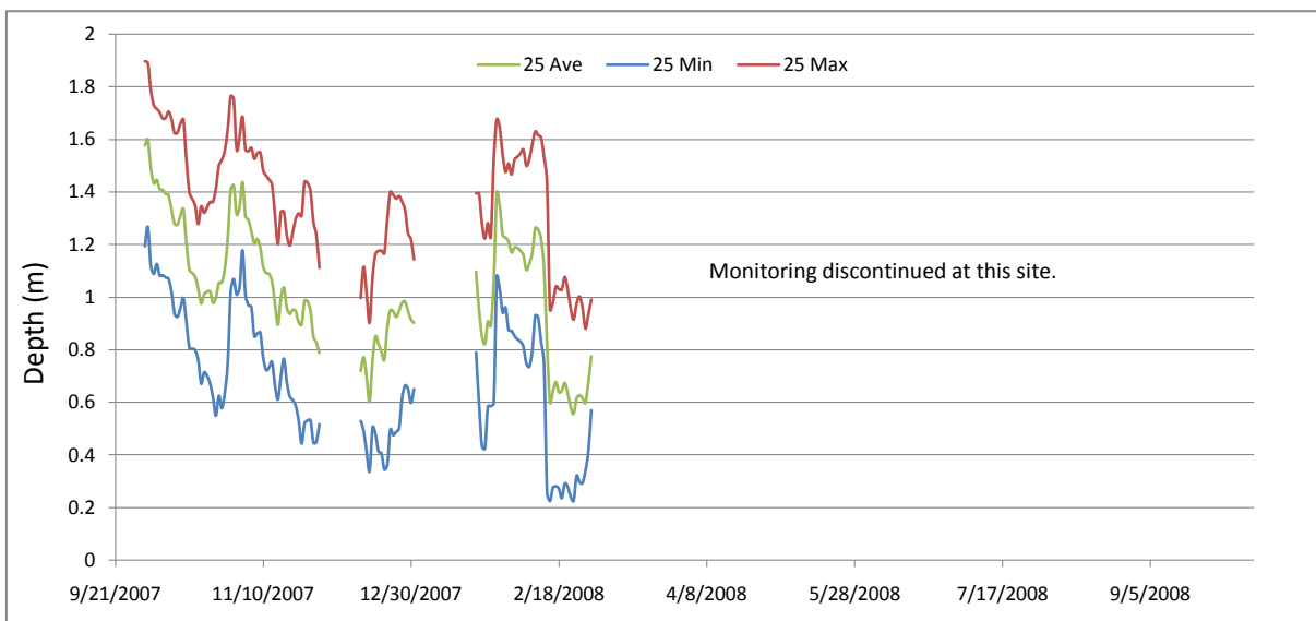
Station 25 daily average, minimum, and maximum of water quality parameters measured by Datasonde recording at 15 minute intervals, Loxahatchee River, Florida. Data not meeting quality control criteria excluded.
