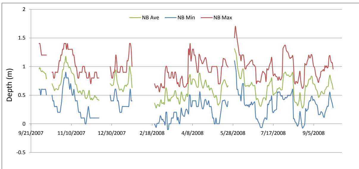
Station North Bay (NB) daily average, minimum, and maximum of water quality parameters measured by Datasonde recording at 15 minute intervals, Loxahatchee River, Florida. Data not meeting quality control criteria excluded.
